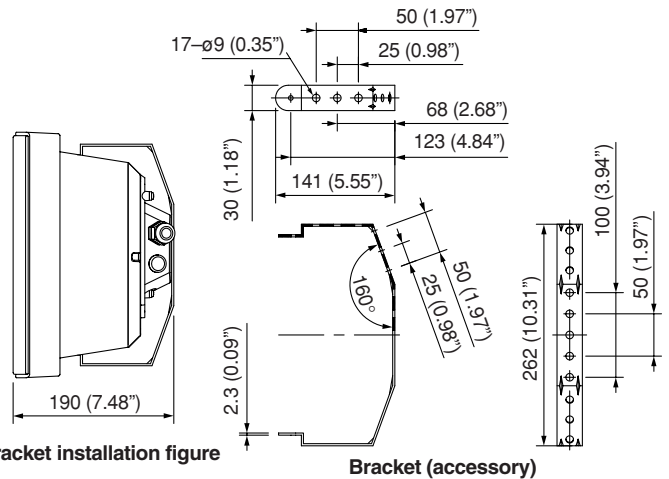
Bracket (accessory)
