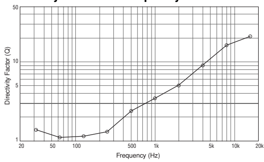
Directivity Factor vs. Frequency
