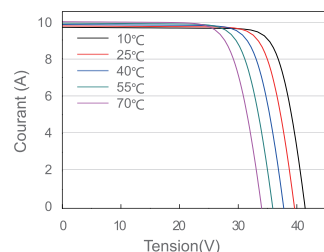
Courbe courant-tension JAM60S02-300/PR
