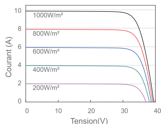
Courbe courant-tension JAM60S02-300/PR
